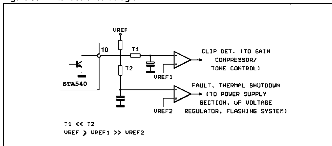
Figure 33. Interface circuit diagram
