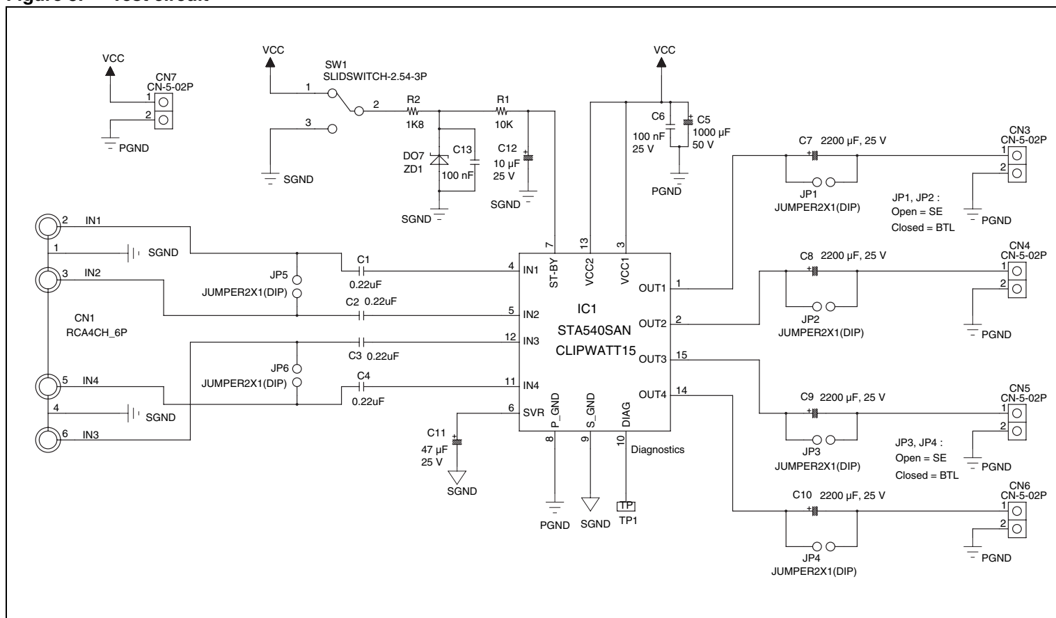
Figure 3. Test circuit
