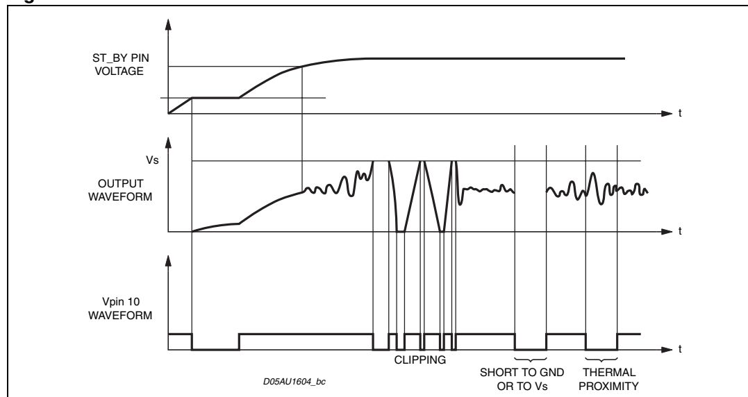
Figure 32. Waveforms
