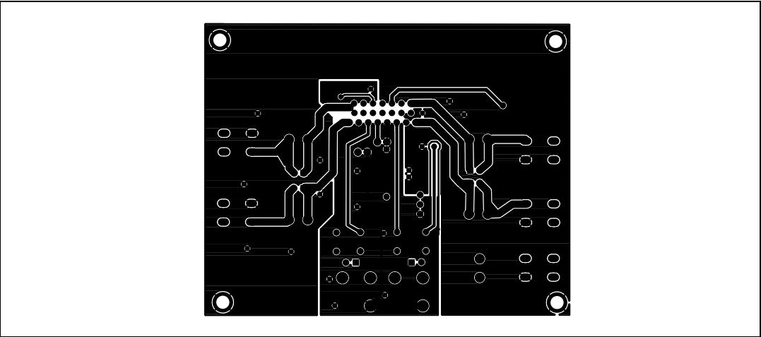
Figure 6. Solder side
