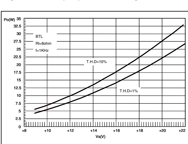
Figure 21. Output power vs voltage
