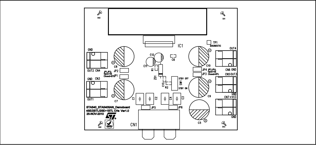
Figure 5. Component side
